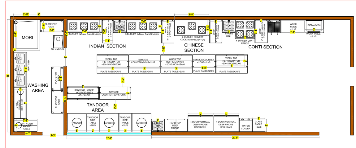
KITCHEN LAYOUT
