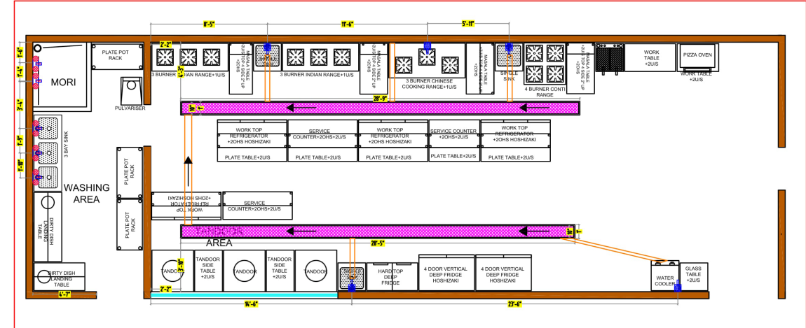
PLUMBING LAYOUT
