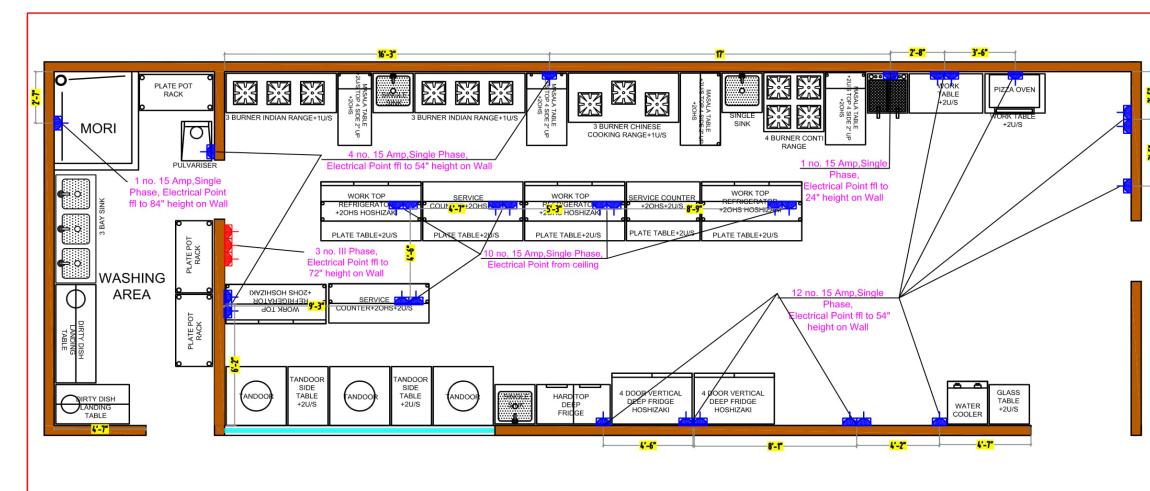
ELECTRICAL LAYOUT
